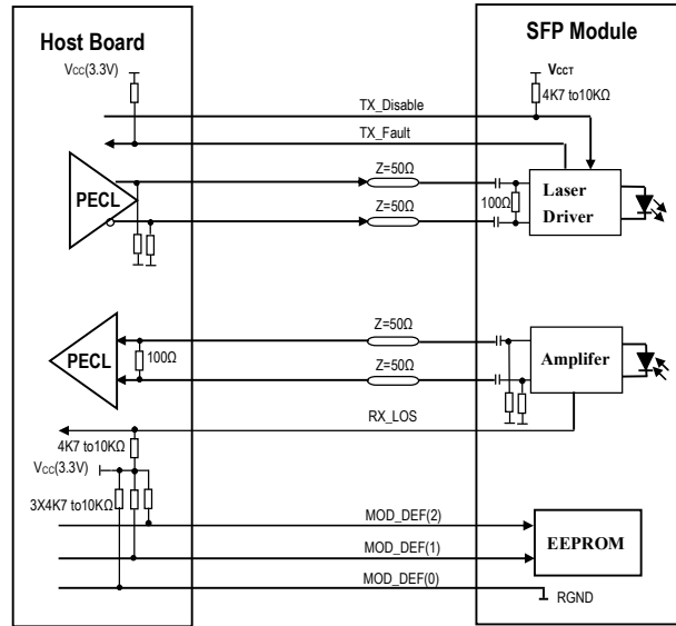
CWDM SFP Host Recommended Circuit
