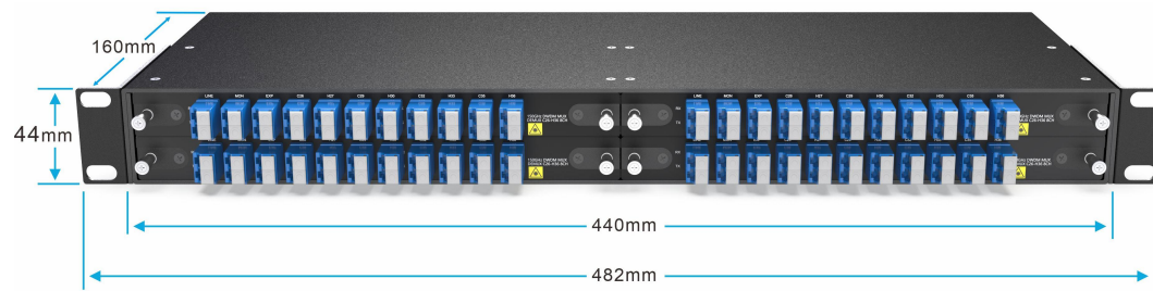
4-Slot 1U Rack for LGX BOX
