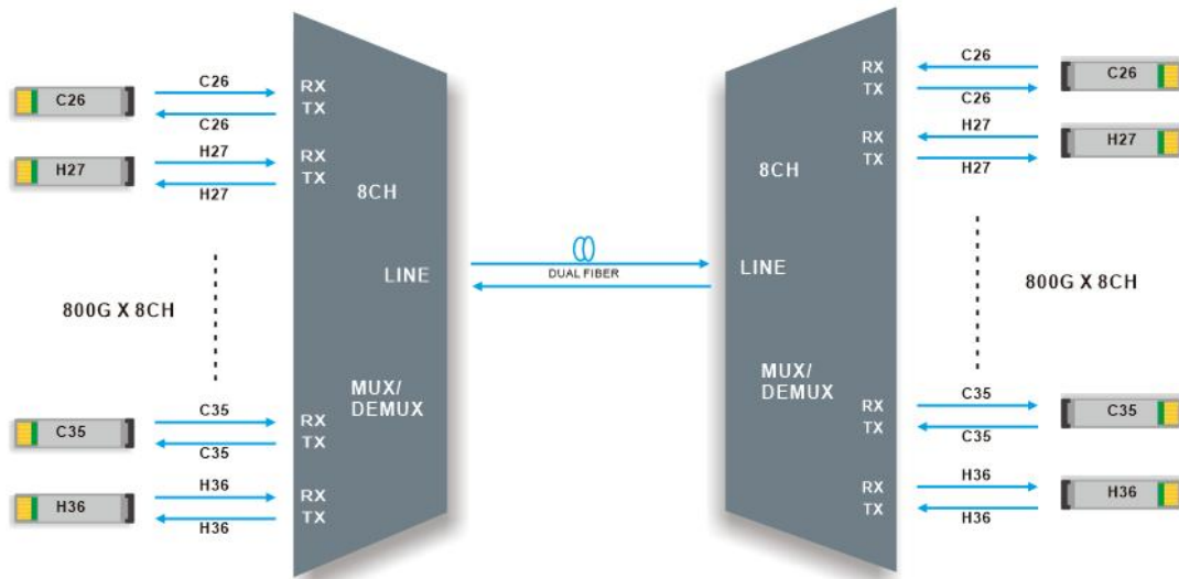
8CH DWDM MUX DEMUX Dual fiber transmission
