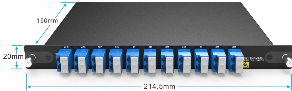
LGX BOX Plug in 4-Slot 1U Rack
