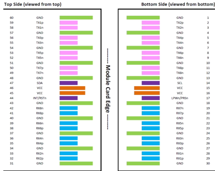
Electrical Pin-out Details for OSFP
