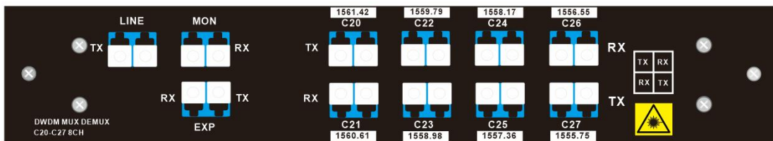
8CH DWDM MUX DEMUX Dual Fiber
