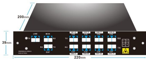
LGX BOX Plug in 2-Slot 1U Rack
